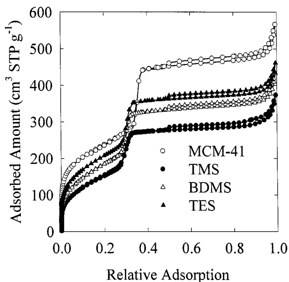
Figure 2. Nitrogen adsorption isotherms for the unmodified MCM-41 and the samples modified with alkylchlorosilanes.
